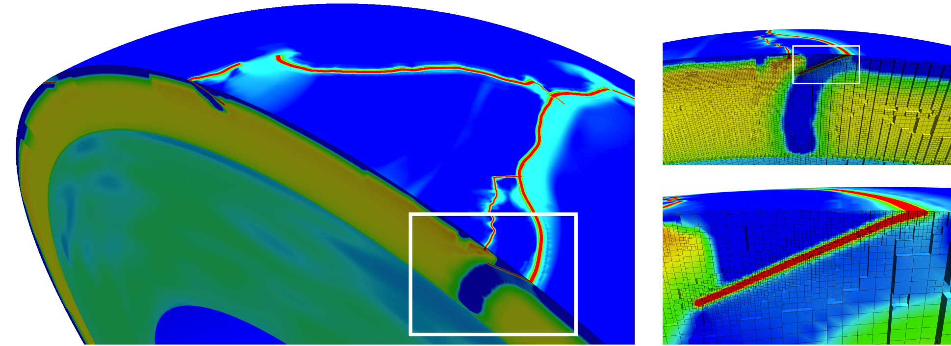
Effective viscosity field and adaptive mesh resolving narrow plate boundaries (shown in red). (Visualization by L. Alsic)
